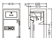
PSG-125EV ¥681,000 (税別) PSG-125EVR 納 ¥710,000 (税別)
