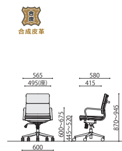
PLC-110L
