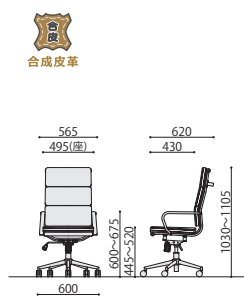
PLC-110H
