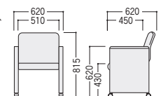
MC-591DFC
