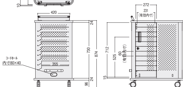
TNC-20PC
