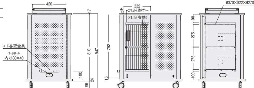
TNC-44SPC
