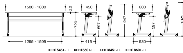
KFH1545T-□ KFH1560T-□ KFH1845T-□ KFH1860T-□
