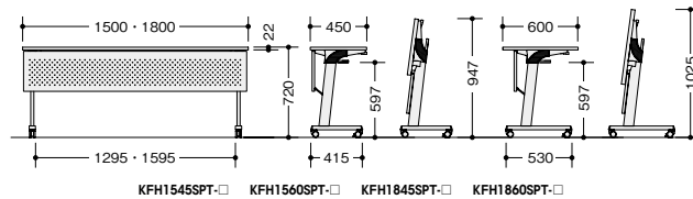
KFH1545SPT-□ KFH1560SPT-□ KFH1845SPT-□ KFH1860SPT-□
